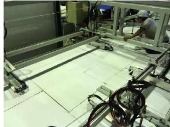
Automatic Cutting and Sealing machine
